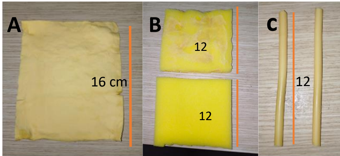
Figure 1. Preparation of the phantom. A: polyvinyl alcohol sheet 16x16 cm in size. B: polyurethane sponge 12x12 cm in size. C: Urinary catheter trimmed to 12 cm.
